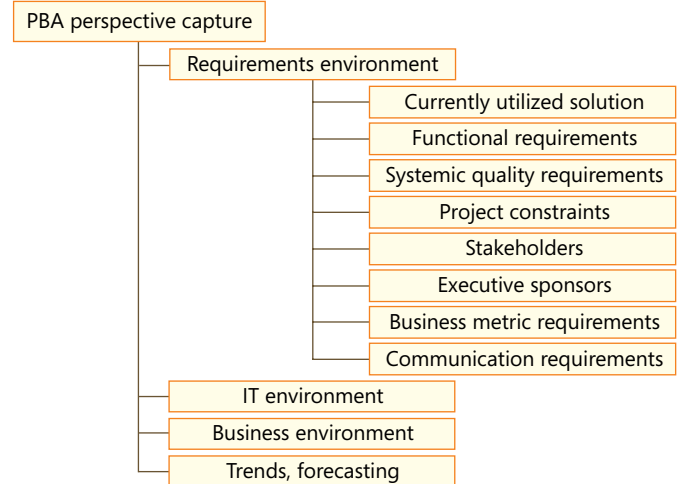
Figure 4 The requirements environment
