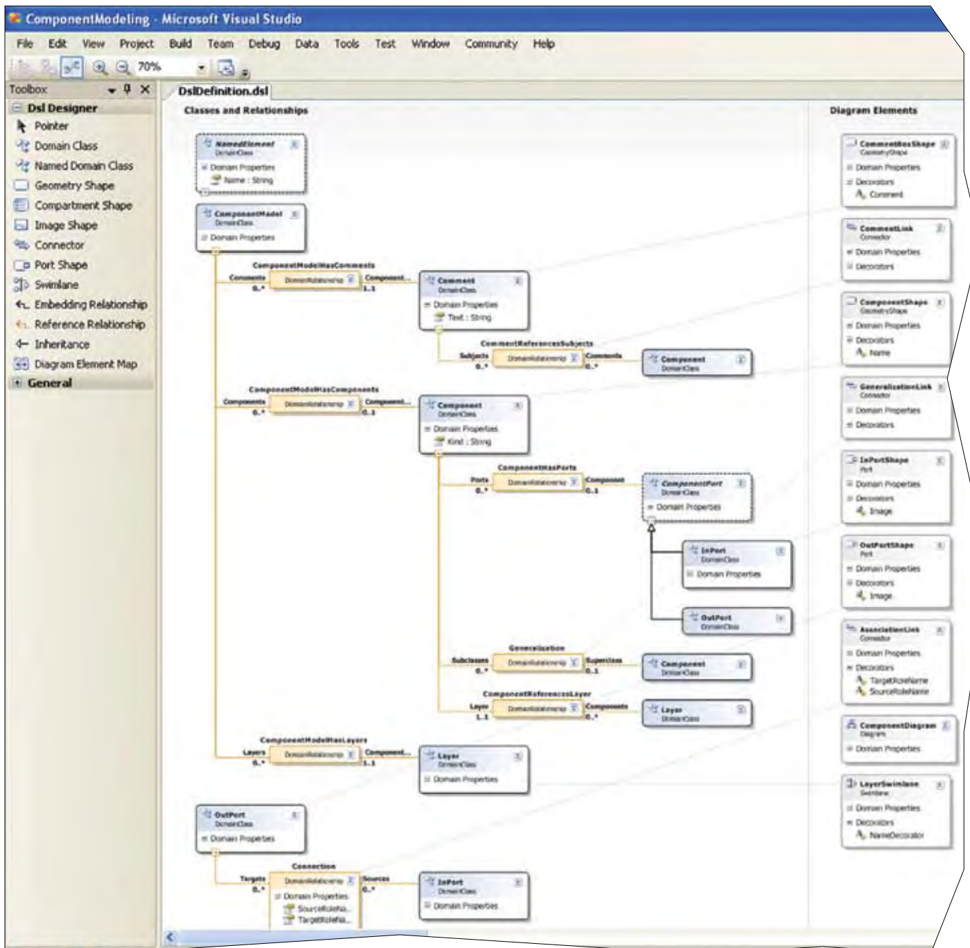
Figure 6 Swimlanes added to the DSL definition
