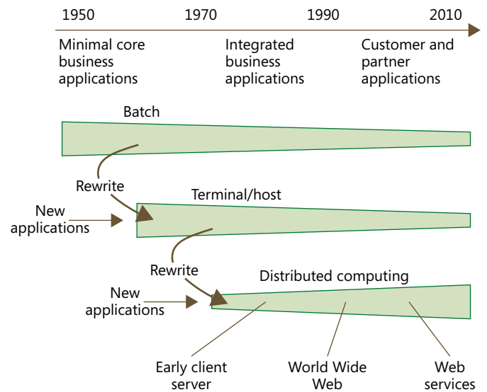
Figure 1 Time-phased trending in application architecture patterns
